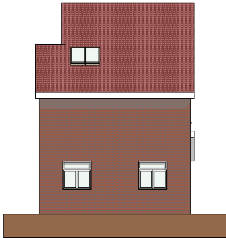
Rear Elevation (West) Elevation 1:100
